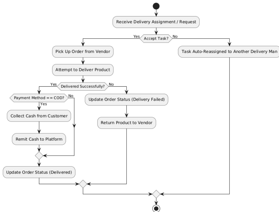
Delivery Man Activity Diagram
