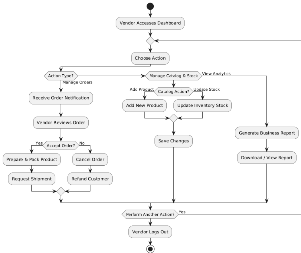
Vendor Activity Diagram
